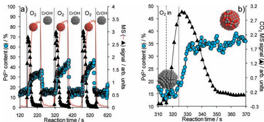
Figure 3. (a) MS/XANES intensities during alternating CrOH/O 2 cycles over the 2.37 wt % Pd/mesoporous Al 2 O 3 catalyst at 250 °C: red line, O 2 ( m/z 32); ▲, CO 2 ( m/z 44); blue ●, fitted XANES Pd 2+ concentration. (b) Evolution of CO 2 yield and Pd oxidation state during CrOH/He → O 2 /He switchover of the reactant stream over the 2.37 wt % Pd/mesoporous Al 2 O 3 catalyst at 250 °C. Combustion occurs before reoxidation of metal nanoparticles.
